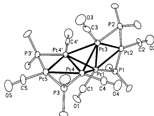
Figure 1. Molecular structure of 2 2+ . [7] Methyl groups are omitted for clarity (thermal ellipsoids at 30 % probability; symmetry code: ' = x, -y, z). Selected bond lengths [Å] and angles [°]: Pt1-Pt2 2.758(1), Pt1-Pt3 2.667(1), Pt1-Pt4 2.841(1), Pt2-Pt3 2.762(1), Pt3-Pt4 2.841(1), Pt4-Pt4' 2.666(1), Pt4-Pt5 2.756(1); Pt3-Pt1-Pt2 61.17(3), Pt1-Pt2-Pt3 57.79(3), Pt1-Pt3-Pt2 61.04(3), Pt3-Pt1-Pt4 62.00(3), Pt1-Pt3-Pt4 62.00(3), Pt1-Pt4-Pt3 56.00(3), Pt1-Pt4-Pt4' 62.01(2), Pt3-Pt4-Pt4' 62.01(2), Pt4'-Pt4-Pt5 61.071(15), Pt4-Pt5-Pt4' 57.86(3).
